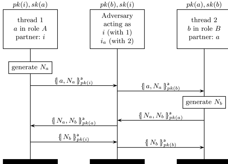
Fig. 24.2. Lowe's man-in-the-middle attack on the Needham-Schroeder protocol
